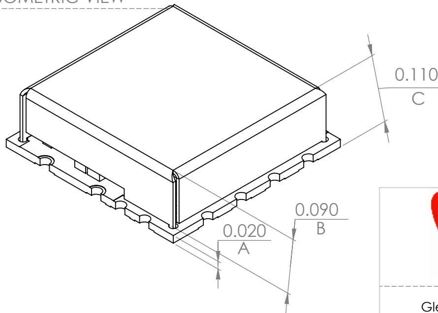
ISOMETRIC VIEW
