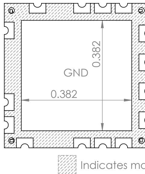
BOTTOM VIEW - BOTTOM SIDE
